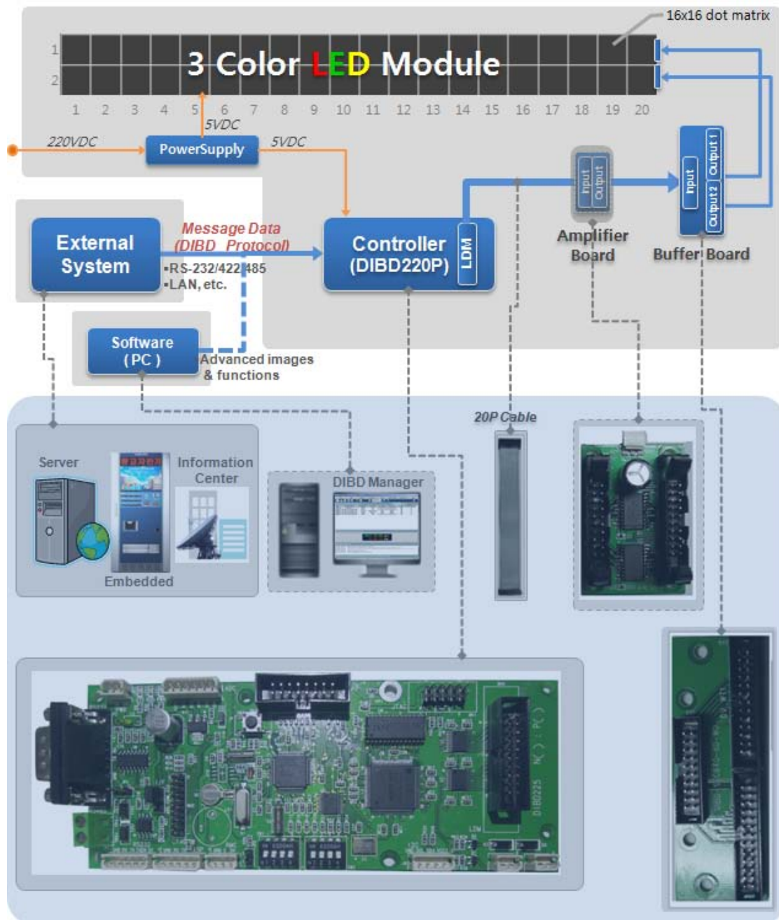
Fig. 1 Configuration of 3 Color LED sign with DIBD220P
