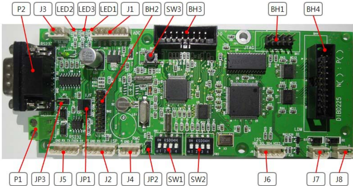
Fig. 2 DIB220 of 3 Color LED Sign Controller
